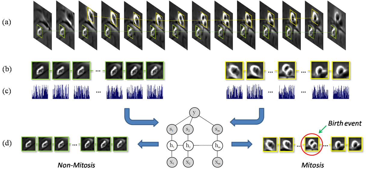
Fig. 1. Summary of the mitosis detection procedure. (a) Candidate patch sequence extraction from consecutive phase-contrast microscopy image frames. (The original images are much larger than these examples.) (b) Examples of candidate patch sequences. (c) Unique scale gradient histograms computed for each patch in candidate patch sequences. (d) Identification of mitosis occurrence and temporal localization of a birth event using Event Detection Conditional Random Field (EDCRF).
